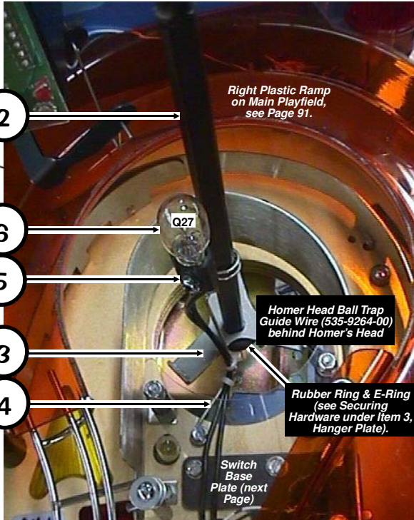
Assembled View ▼
